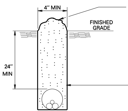
1 SECONDARY, SERVICE, OR STREET LIGHT CONDUIT
